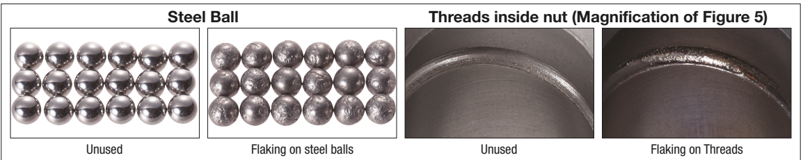
Figure 6 Flaking on Ball Screw Components
